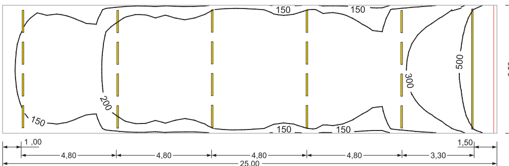
ilia-ILG/1200 4000lm
